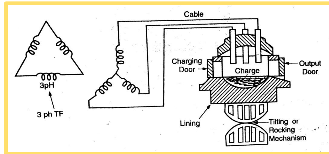
(3-Phase direct Arc Furnace)
